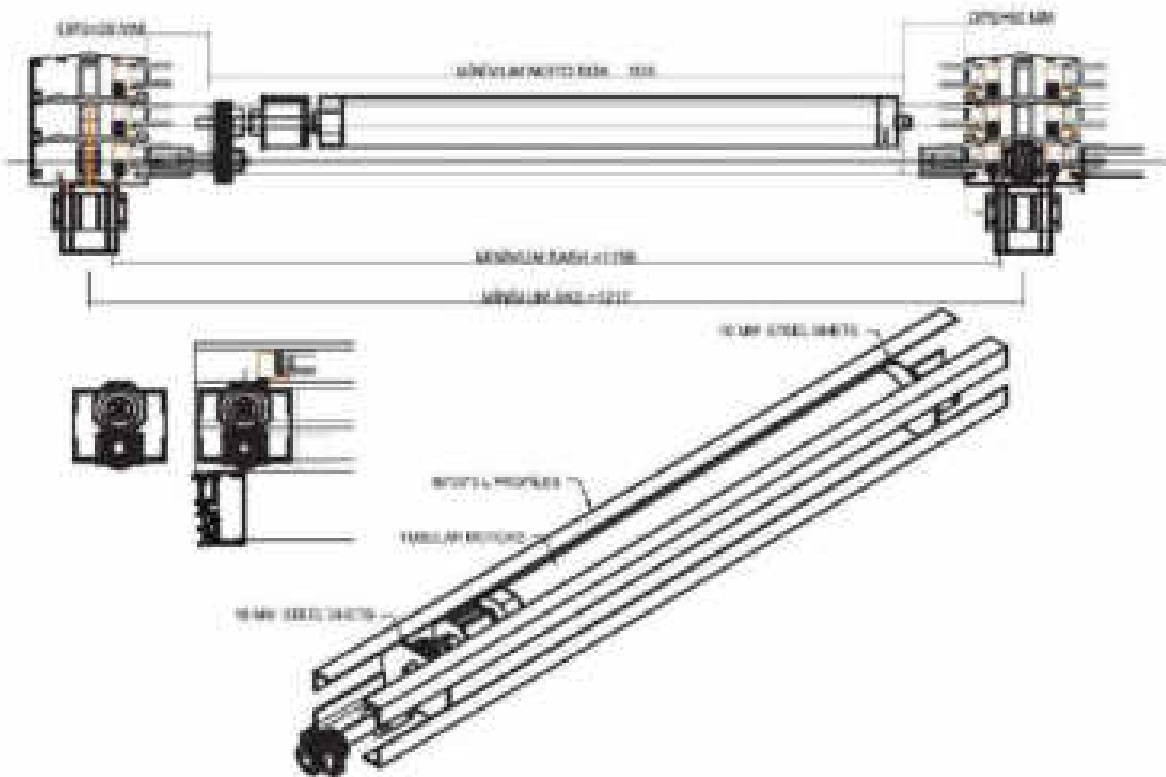
120 NM TUBULAR MOTOR DETAILS
