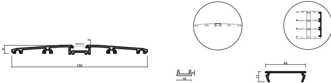
580-1204 ( 1,450 kg/mt ) SRA150M06 DUVAR BİTİM PROFİLİ
