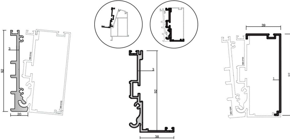
580-1204 ( 1,450 kg/mt ) SRA150M06 DUVAR BİTİM PROFİLİ
